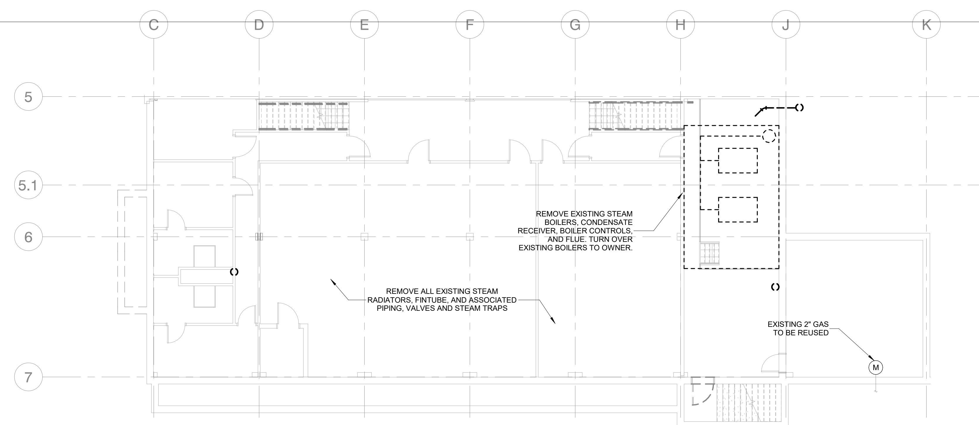
2 HVAC BUILDING 1 BASEMENT DEMO PLAN 1/8" = 1'-0"
